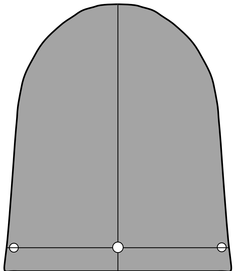
Tool for checking level of wing spar.
